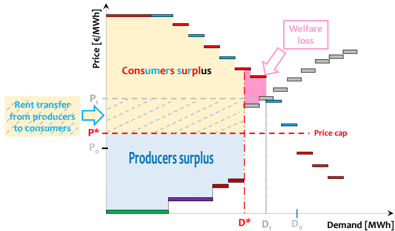
Figure 9: Impact of a windfall profit tax implemented as a price cap.
