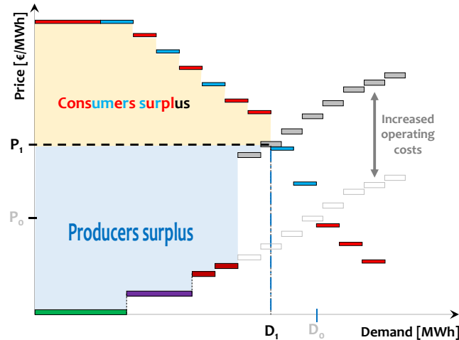
Figure 8: Impact of increased operating costs of the marginal unit on the clearing price and welfare under perfect competition.
