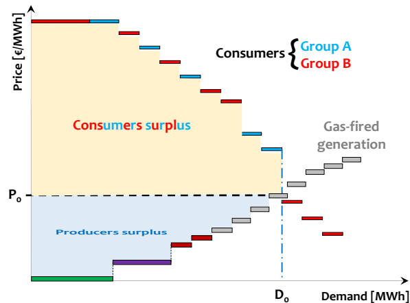
Figure 7: Marginal pricing clearing.
