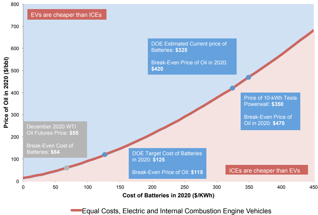
Figure 6: Break-even oil and battery costs
