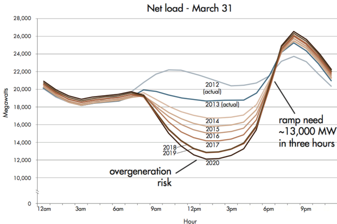
Figure 5: California ISO's "Duck Curve"
