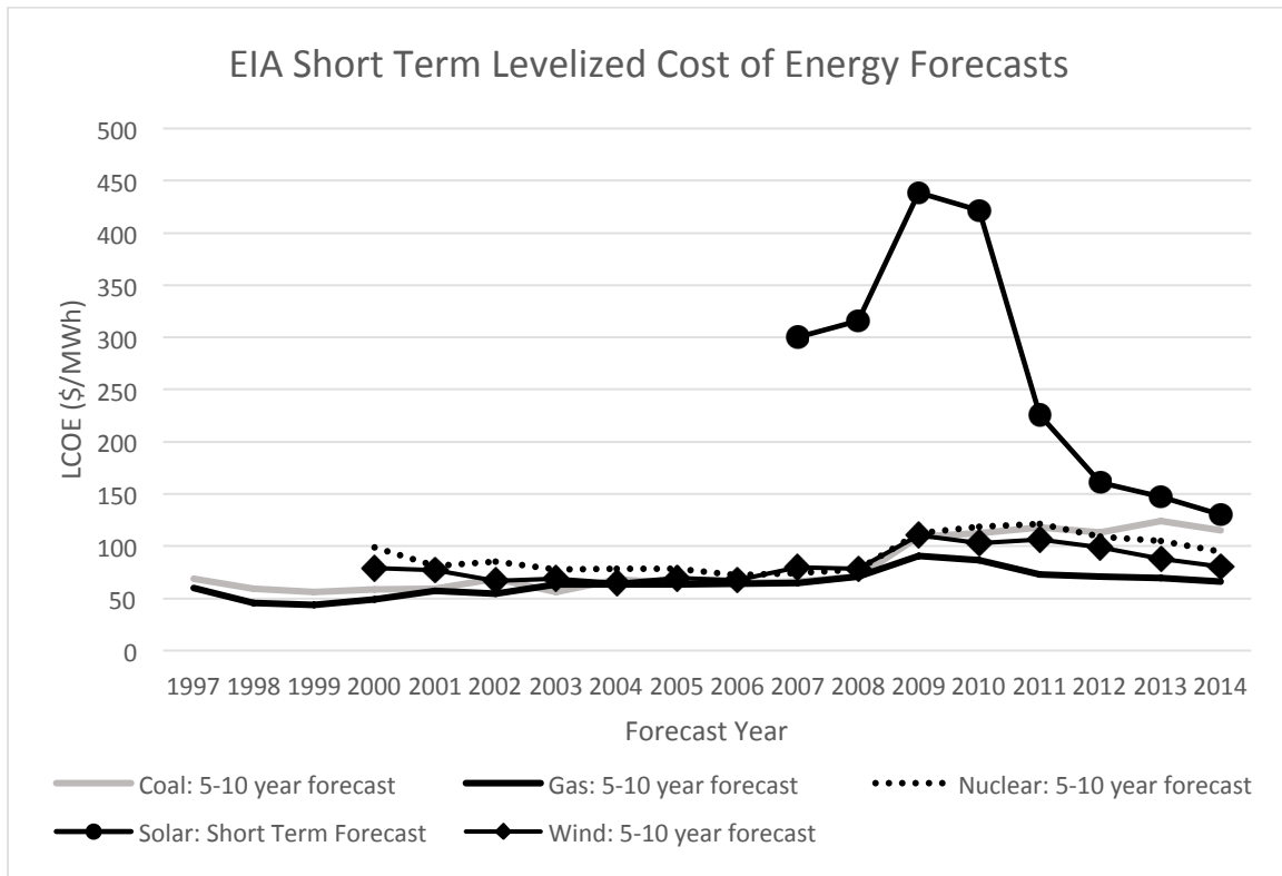
Figure 4: Levelized Cost of Energy forecasts from EIA Annual Energy Outlook reports from 1997-2014
